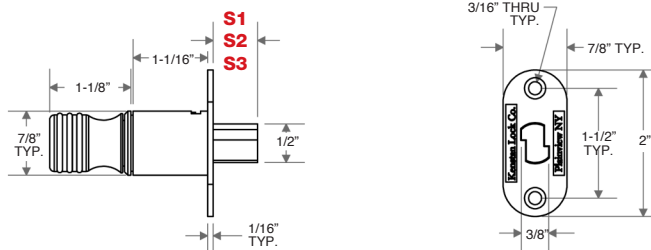
All dimensions shown are in the locked position.
